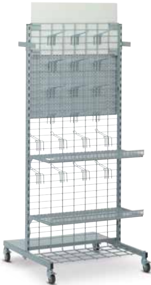
UNIVERSAL Double-sided, mobile chassis with wire shelves, rear panel made of perforated sheet metal, top sign and blister pack double hooks
