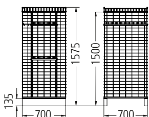
Fig.: POSmodul 7/7 (Module 2) with accessories: wooden pallet, cover plate and basket attachment
