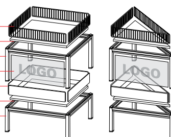
Assembled in a flash: version with mobile module.
