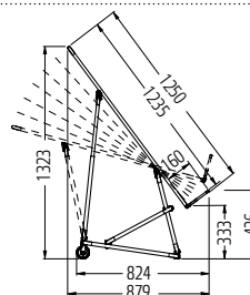
MOBILO - 3 IN A ROW plastic powder-coated, black
