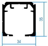
CARRIL SUPERIOR RAIL EN ALUMINIUM ALUMINIUM RAIL BINARIO IN ALLUMINIO 5111/30. 3M
