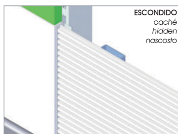
1651/1.. REMATE ÁNGULO 20X20 profil lateral de finition lateral finishing profile profilo laterale di finitura
